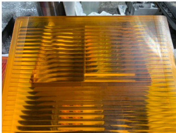
Acrylic plastic cut with FCLP Freedom cutter with a single PCD tipped insert.
