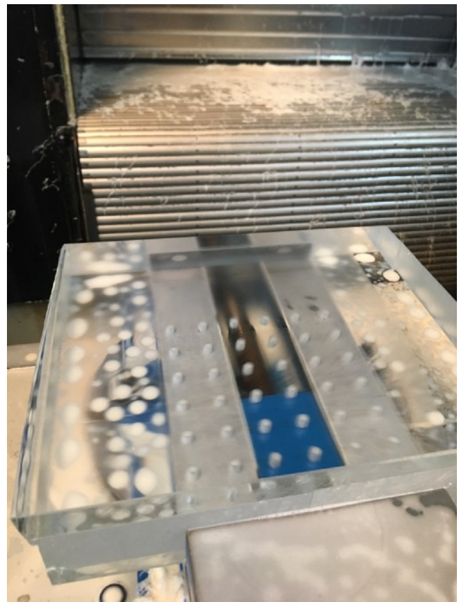
Acrylic plastic cut with FCLP Freedom cutter with a single PCD tipped insert.
